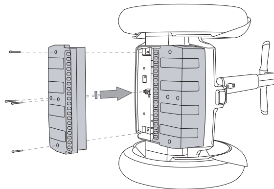
Figure 10: Torque the two center fasteners first.
