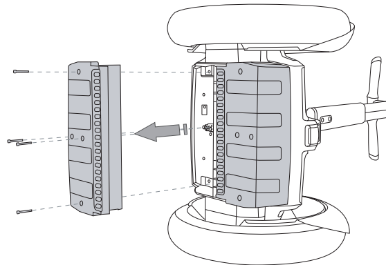
Figure 66: Remove the Batteries
