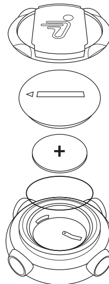
Figure 76: Replacing the InfoKey Controller Battery
