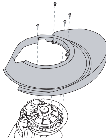
Figure 70: Remove/Install the Fenders
